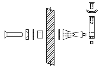
EXPLODED VIEW
