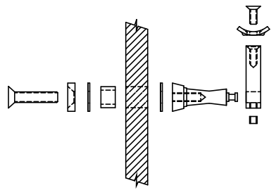
EXPLODED VIEW
